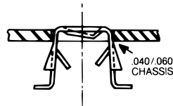
PART ENTERS CHASSIS FROM BOTTOM SIDE
